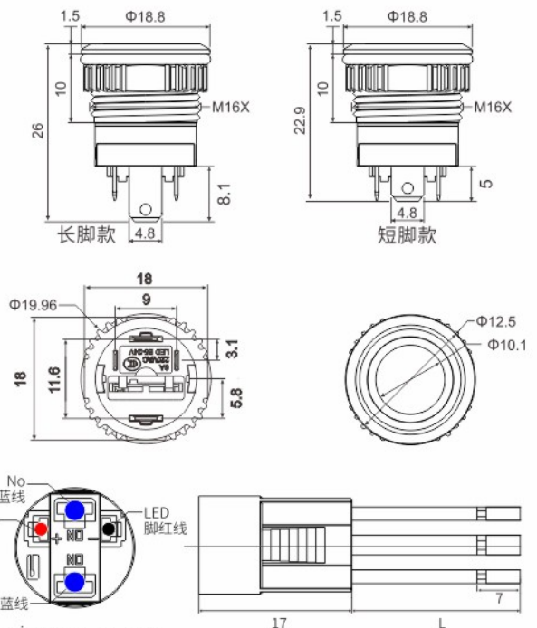
镀银长插脚 Silver Long Plated Pins
