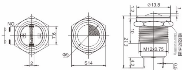
12B外形尺寸 Outline Dimension
