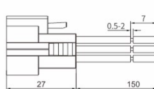
头部防水,高亮LED IP65, With LED
