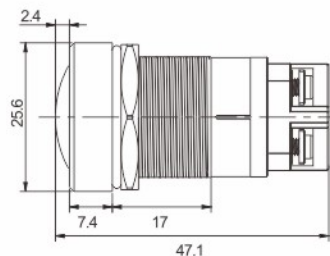
螺丝脚方便接线 Screw Pins
